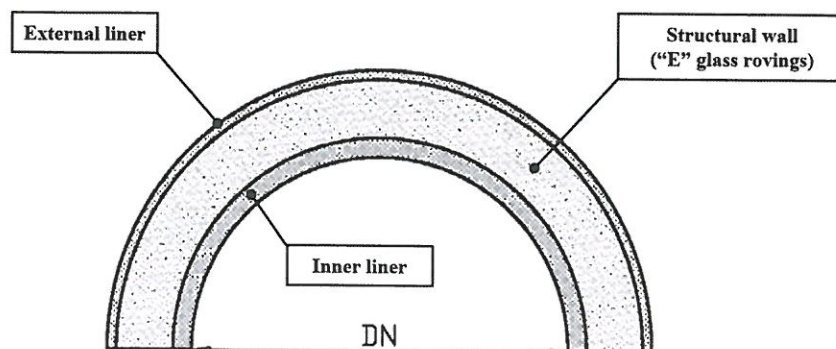
Figure 1: FW pipes wall section.
